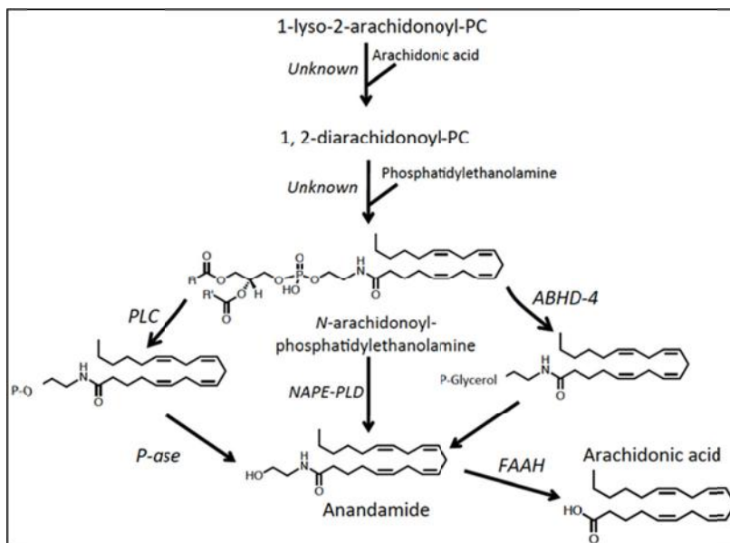
FIGURE 2-3 Pathways of anandamide formation and deactivation.
